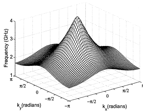
Fig. 3. Dispersion characteristic of L - C dual TL network.
